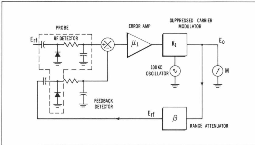
Fig. 6. Circuit arrangement of -hp- 411A RF Millivoltmeter. Feedback detector diode and rf detector diode have matched temperature characteristics and are located together in probe in thermal proximity to minimize drifts caused by thermal changes.
