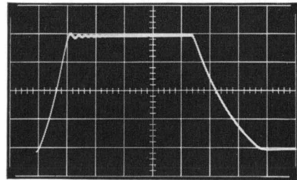
Fig. 4. Response at 411A output terminal to a full-scale burst of rf applied to 411A input. Sweep time is \frac{1}{2} sec/cm; vertical scale is \frac{1}{4} -volt/cm.
