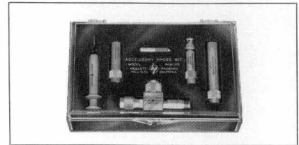
Fig. 11. Accessories are available as a kit (411A-21G) which also includes spare set of matched detector diodes.
