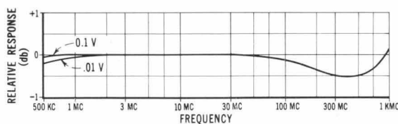
Fig. 7. Typical frequency response of -hp- 411A RF Millivoltmeter as used with -hp- 411A-21D Type N Tee. 411A can also be used as voltage indicator to about 3 1/2 kmc, since beyond 1 kmc frequency response characteristic typically exhibits a resonant rise of several db, peaking at about 2 1/2 kmc.
